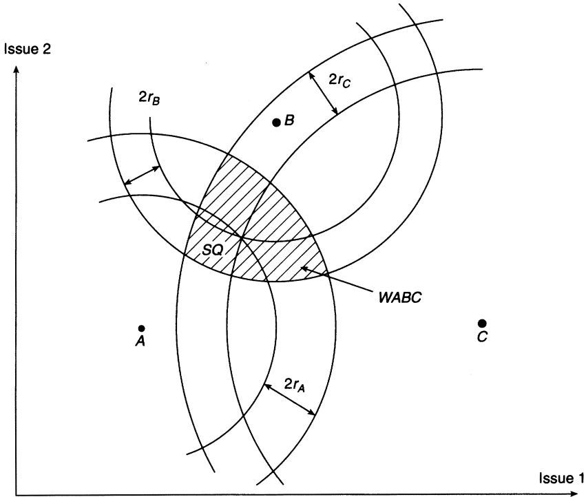
Status quo cannot be replaced if decision makers are individuals; it can be moved anywhere inside WABC if decision makers are collective; r_A, r_B, r_C are the radii of the yolks of players A, B, C .
