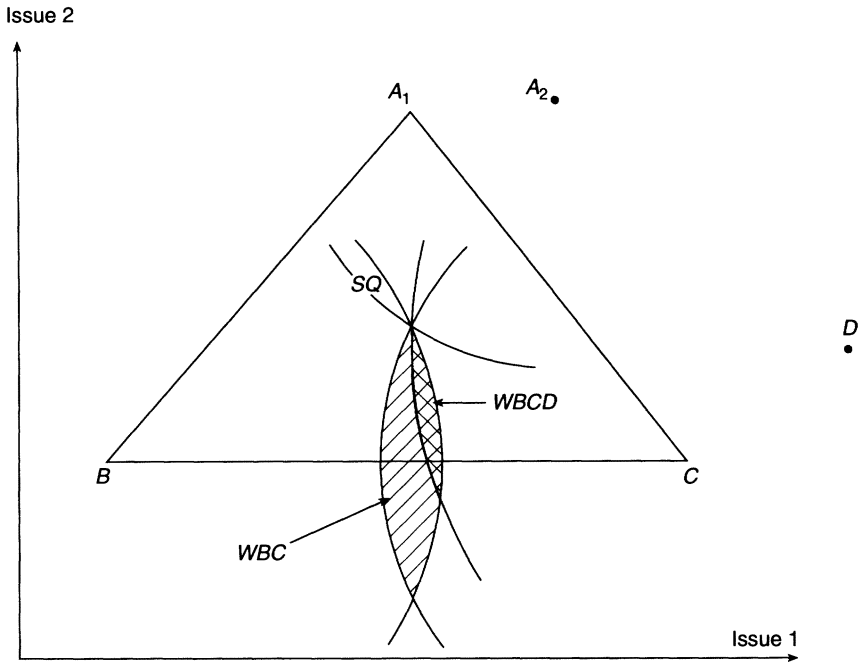
Status quo cannot be changed even if A_1 moves to A_2 . If A_1 is replaced by D , then the status quo can be replaced by any point in the WBCD area.
