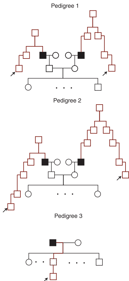
Fig. 3. Illustrations of the three CEU pedigrees (black) showing how genetic information from distant patrilineal relatives (arrow; red, patrilineal lines) can identify individuals. Filled squares represent sequenced individuals. To respect the privacy of these families, only abbreviated versions are presented. The sex of the CEU grandchildren was randomized. The numbers of grandchildren are not given.
